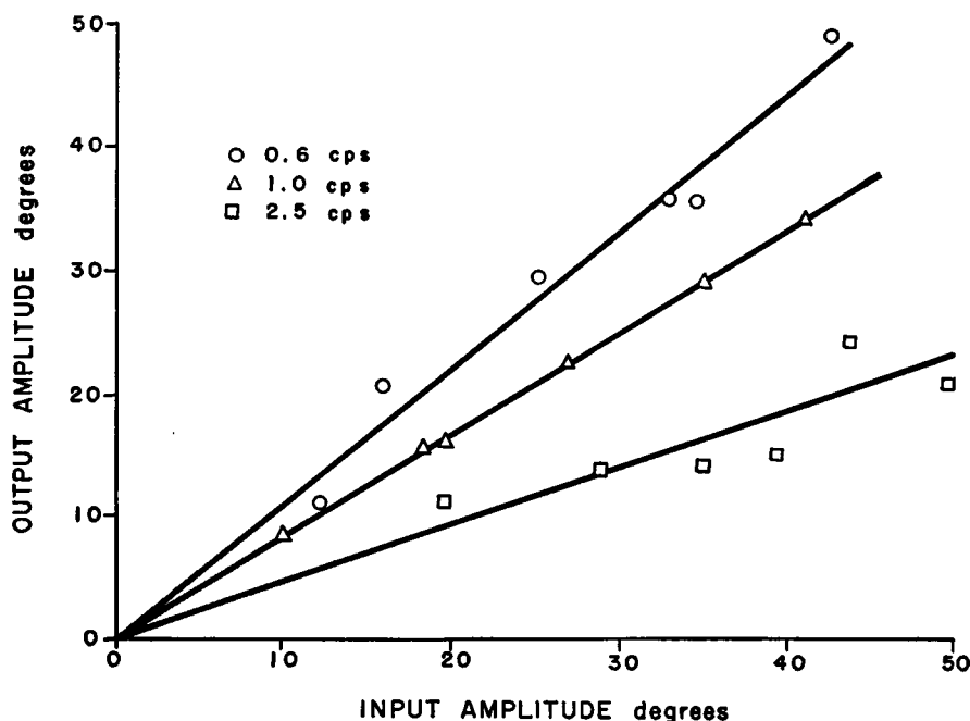
FIGURE 10 Linearity control experiment.
