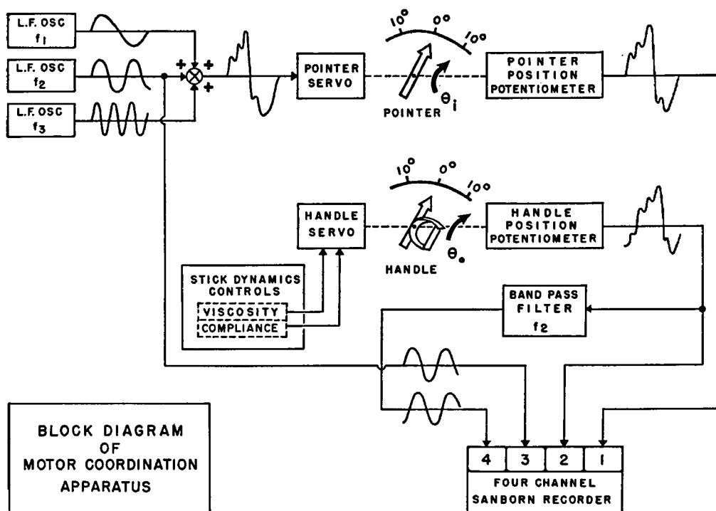
FIGURE 3 Block diagram of motor coordination apparatus.
